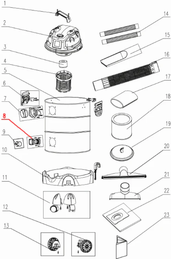
Drain outlet assembly for VQ810SWD
